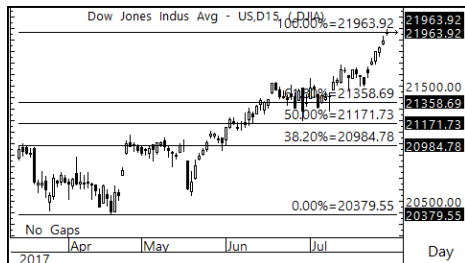
Fibonacci Retracement
